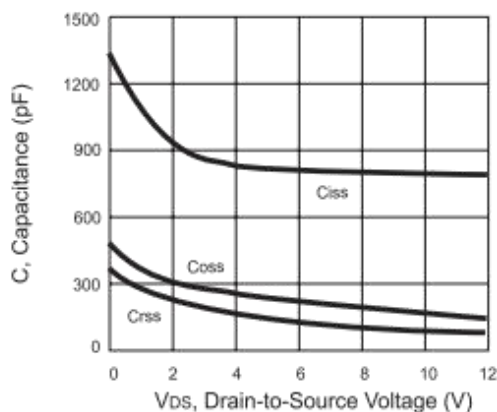
Figure 3. Capacitance
