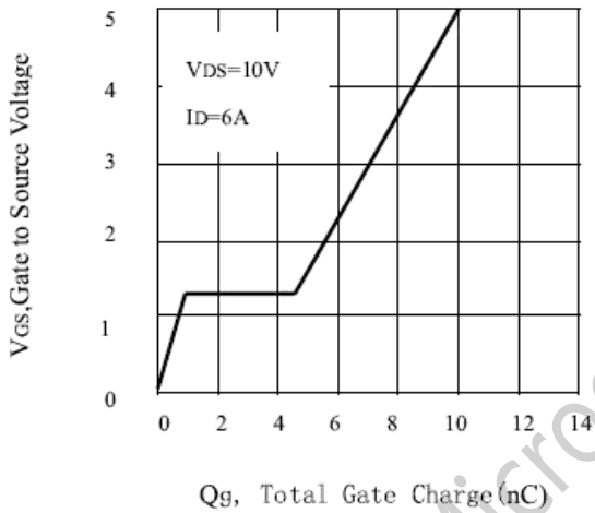
Figure 9. Gate Charge
